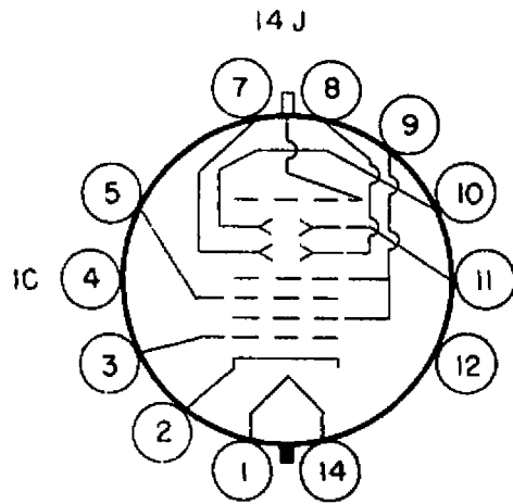
BOTTOM VIEW OF BASE
