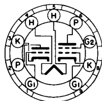
BOTTOM VIEW MINIATURE BUTTON 9 PIN BASE 9FX
