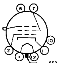
BOTTOM VIEW OF BASE
