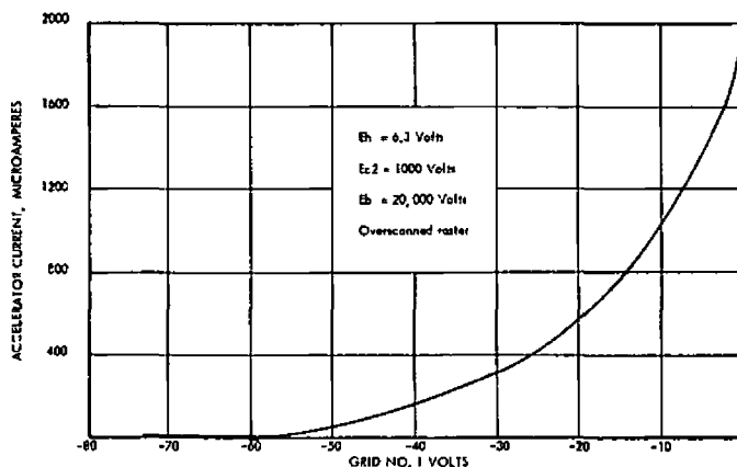
TYPE SCKP- AVERAGE CHARACTERISTICS
