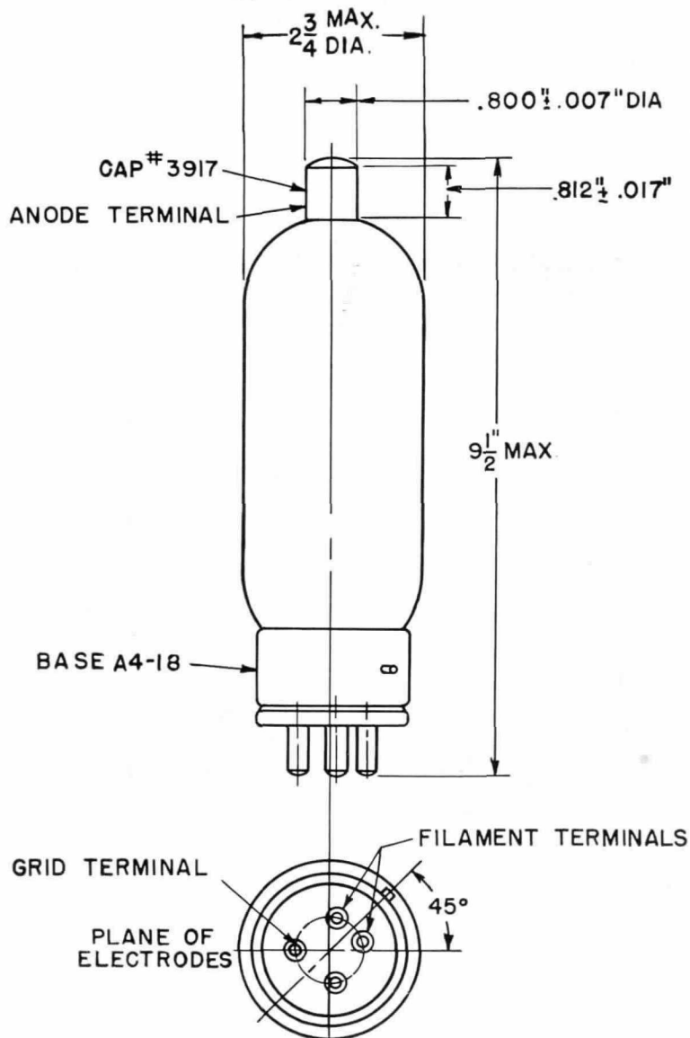
GL-5C24 OUTLINE
