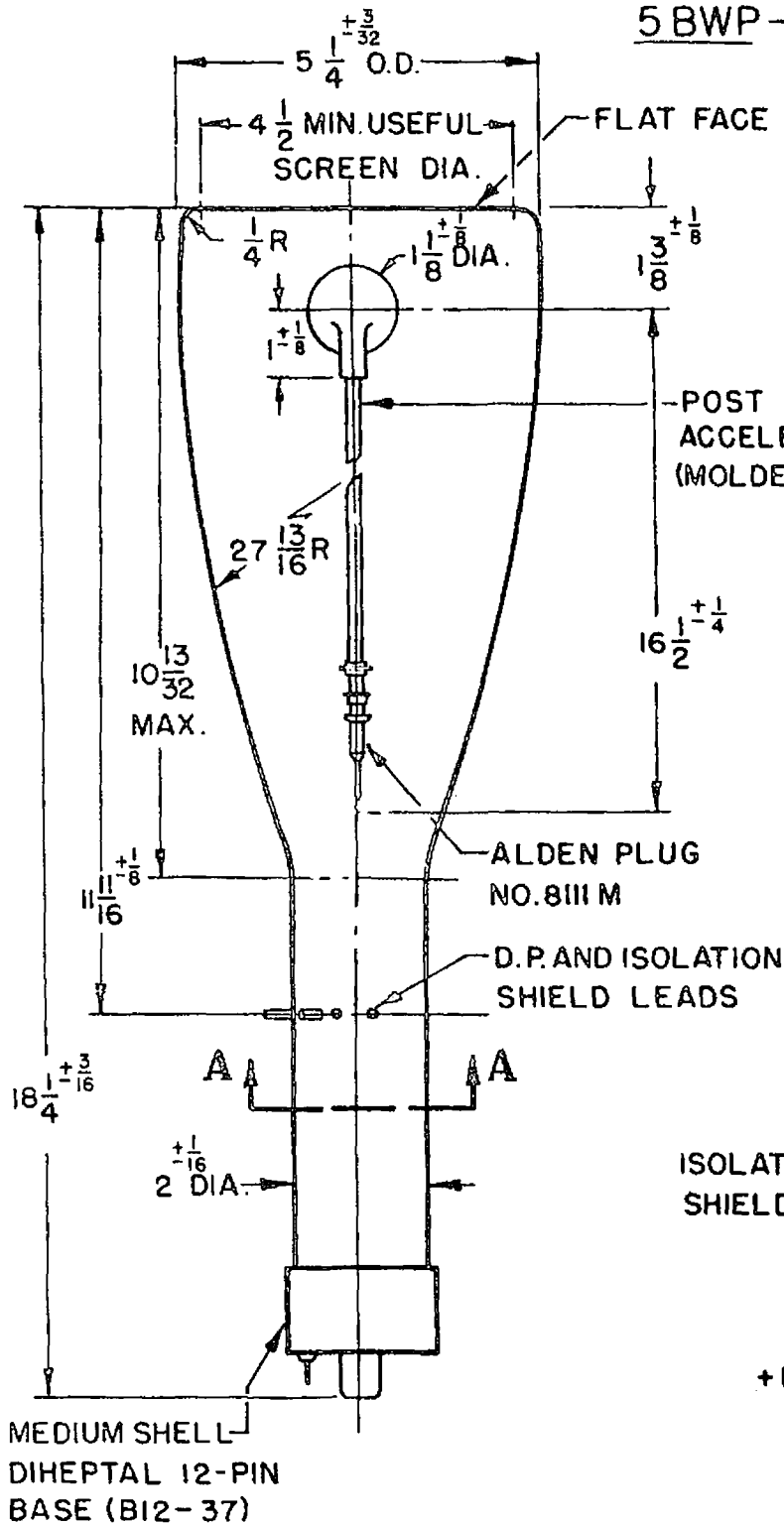
PIN NO. ELEMENT 1 — HEATER 2 — CATHODE 3 — GRID NO. 1 5 — FOCUSING ELECTRODE 9 — ACCELERATOR 12 — DEFLECTION PLATE SHIELD 14 — HEATER CAP — POST-ACCELERATOR
