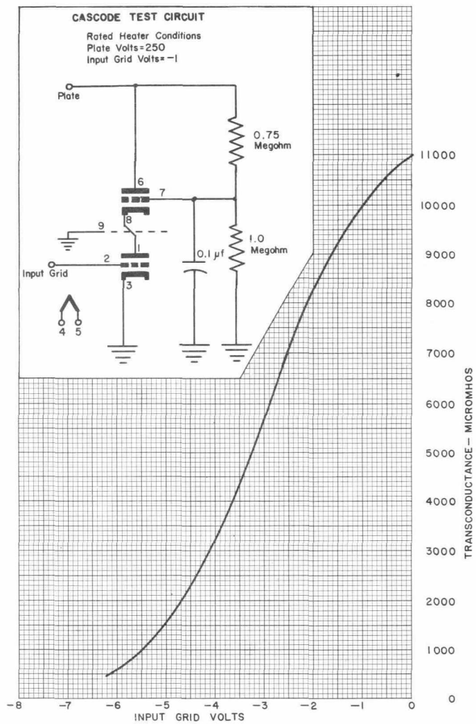
CASCODE TRANSCONDUCTANCE
