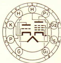
BOTTOM VIEW MINIATURE BUTTON 9 PIN BASE 9FA
