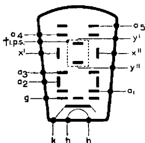
†Inter-plate screen
