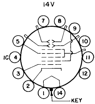
BOTTOM VIEW OF BASE PIN NO. ELEMENT
