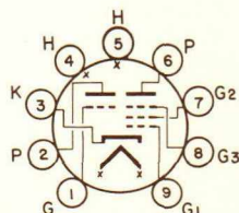
BOTTOM VIEW BASING DIAGRAM JEDEC 9DW
