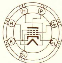
BOTTOM VIEW MINIATURE BUTTON 7 PIN BASE 78Z
