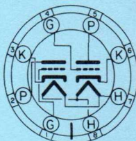
BOTTOM VIEW MEDIUM SHELL 8 PIN OCTAL 880
