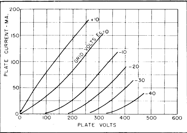
AVERAGE PLATE CHARACTERISTICS TRIODE CONNECTION Ef = 6.3 VOLTS
