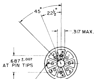
8 PIN INTERMEDIATE SHELL OCTAL BASE
