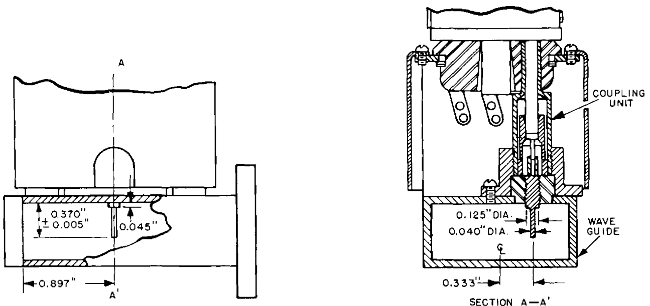
POSITION OF TRANSDUCER COUPLING UNIT WITH RESPECT TO 1\frac{1}{2}'' \times \frac{3}{4}'' WAVEGUIDE
