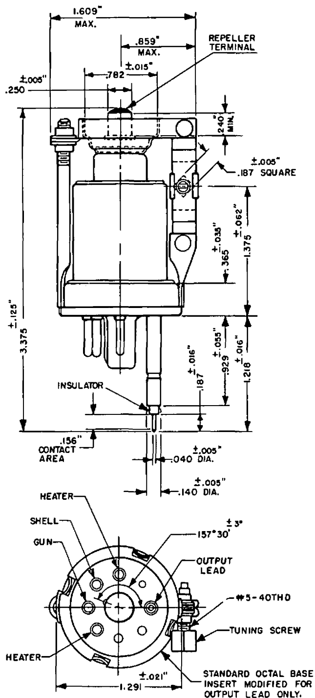
OUTLINE DRAWING
