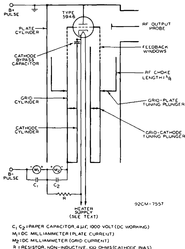
Fig. 3 - Diagrammatic Sketch of Pulsed-Oscillator Circuit of the Folded-Back Coaxial Type Employing the 5946 at 1250 Mc.
