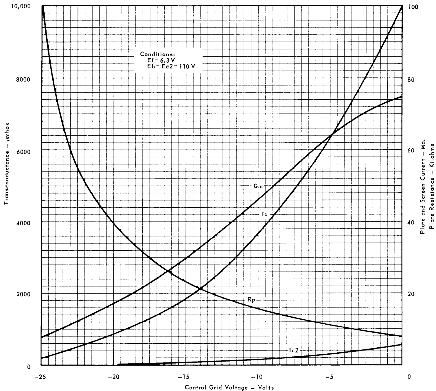
AVERAGE CHARACTERISTICS
