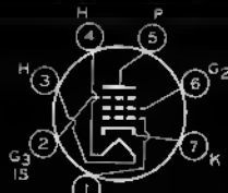
5749 5749/6BA6-W
