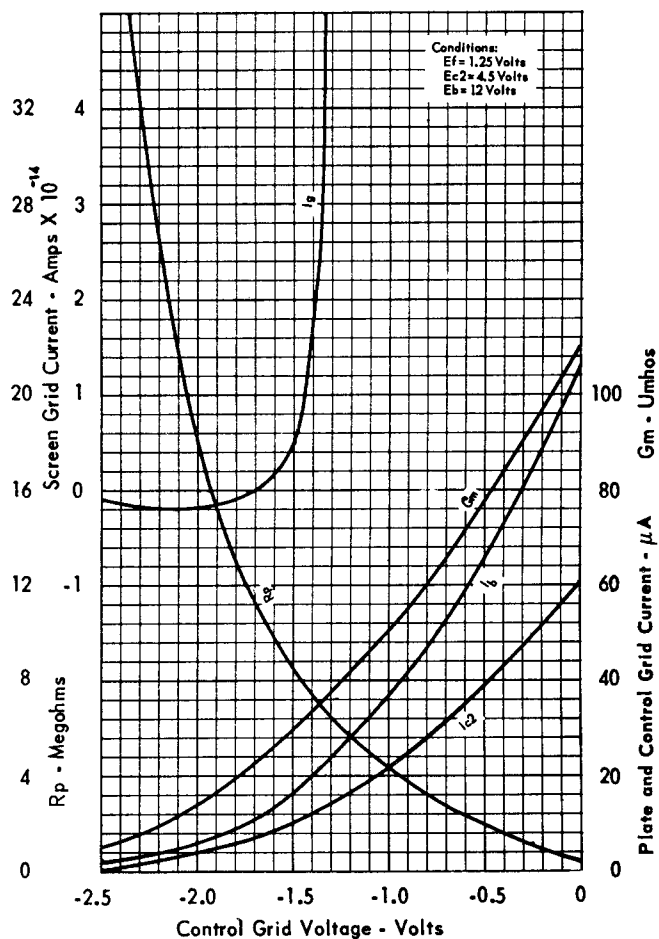
AVERAGE TRANSFER CHARACTERISTICS
