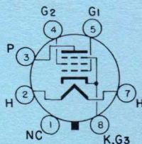
BOTTOM VIEW PINNING DIAGRAM JEDEC 7AC
