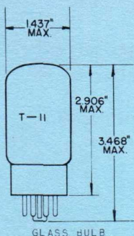
SHORT INTERMEDIATE SHELL 7 PIN OCTAL B7-47 OUTLINE 11-1
