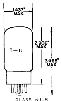
GLASS BULB SHORT INTERMEDIATE SHELL 7 PIN OCTAL B7-47 OUTLINE 11-3
