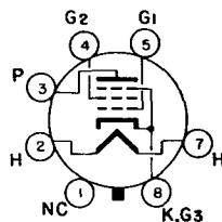
BOTTOM VIEW BASING DIAGRAM JEDEC TAC
