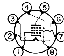
TERMINAL CONNECTIONS: - 8DL
