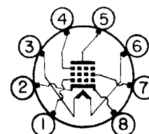
TERMINAL CONNECTIONS: - 8DC
