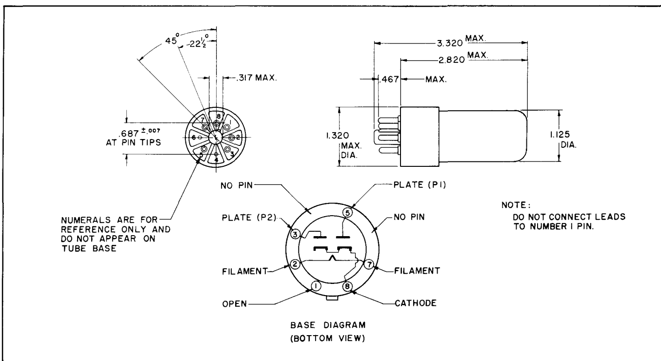
OUTLINE DRAWING
