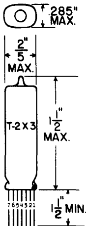
GLASS BULB
