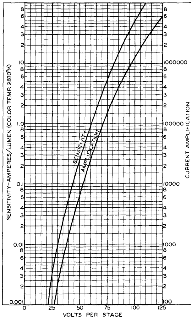
Fig. 3 - Average Characteristics of Type 5819.
