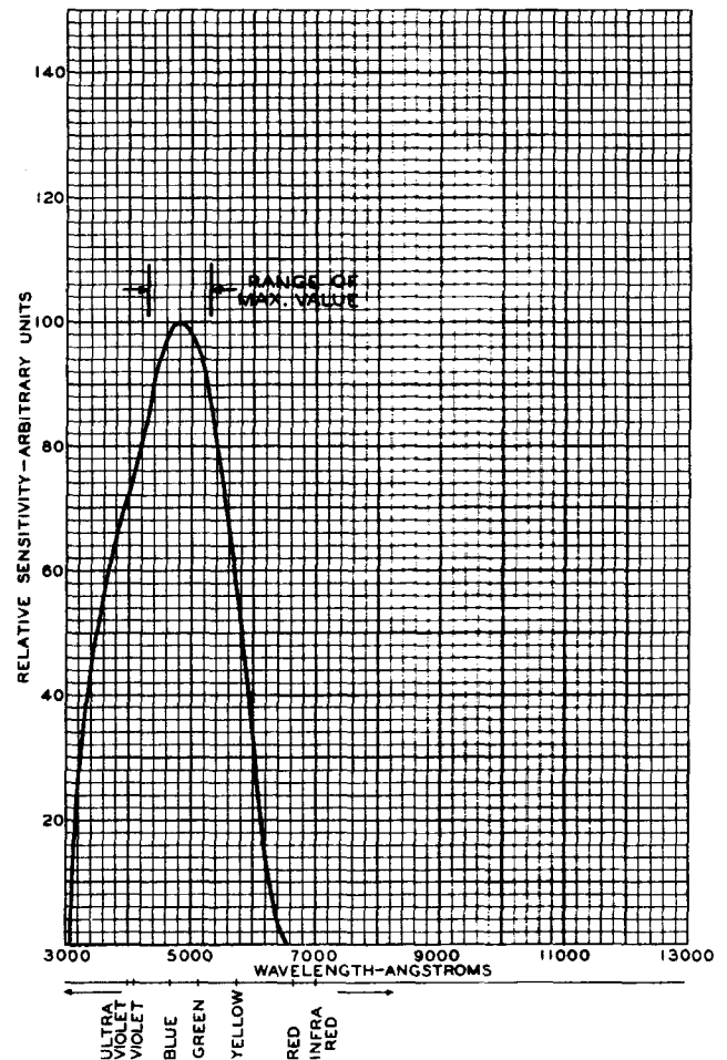
Fig. 1 - Spectral Sensitivity Characteristic of Type 5819 which has S-g Response. Curve is taken for Equal Values of Radiant Flux at all Wavelengths.
