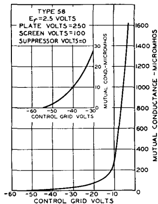
AVERAGE CHARACTERISTICS
