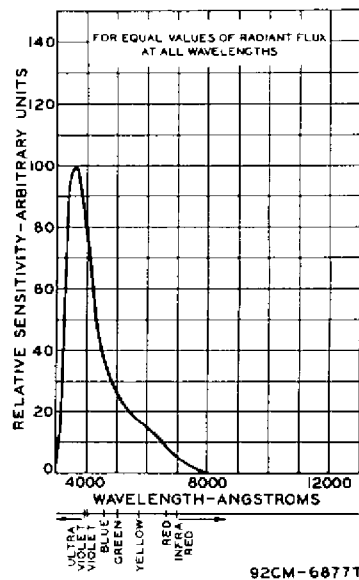
Fig. 6 - Spectral Sensitivity Characteristic of Type 5769.
