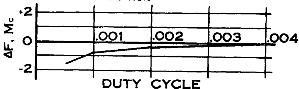
Fig. 7. At 3000 megacycles center frequency, the frequency drift in changing the heater voltages from 5.4 to 7.0 is in the order of 2 megacycles per volt. Likewise, the drift in changing the peak plate voltage from 600 to 1400 is approximately one-half megacycle per 100 volts. The total drift in changing the duty cycle from 0.0005 to 0.004 is in the order of 2 megacycles.
