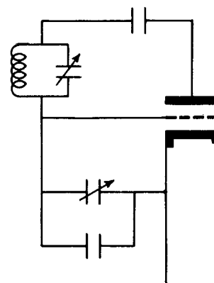
EQUIVALENT CIRCUIT
