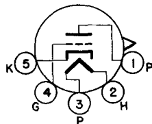
BOTTOM VIEW 0.016" TINNED FLEXIBLE LEADS 0.048" SPACING CENTER-TO-CENTER
