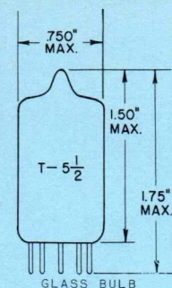
SMALL BUTTON MINIATURE 7 PIN BASE E7-1 OUTLINE DRAWING JEDEC 5-1
