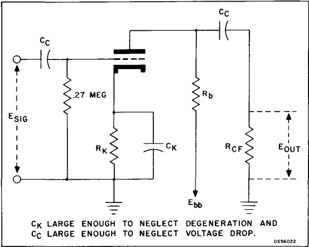
Resistance coupled amplifier circuit.
