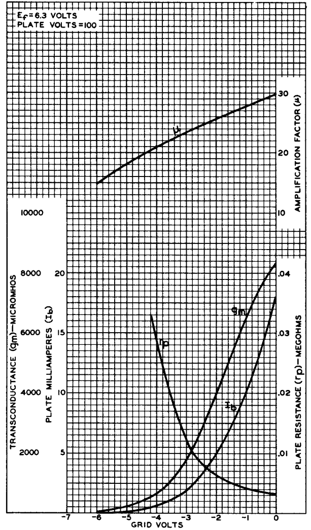
Fig. 2 - Average Characteristics of Type 5718.
