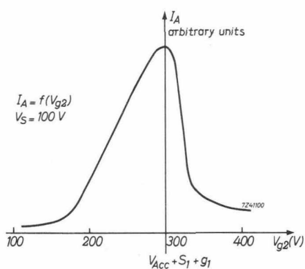
Fig. 6. Anode current variation with the adjustment of g_2 .
