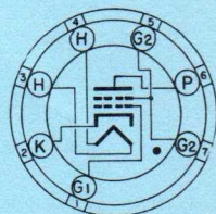
BOTTOM VIEW MINIATURE BUTTON 7 PIN BASE 7BN
