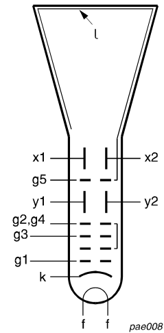
Fig.3 Electrode configuration.
