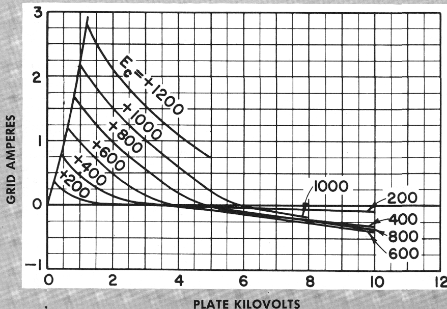
GRID CHARACTERISTICS
