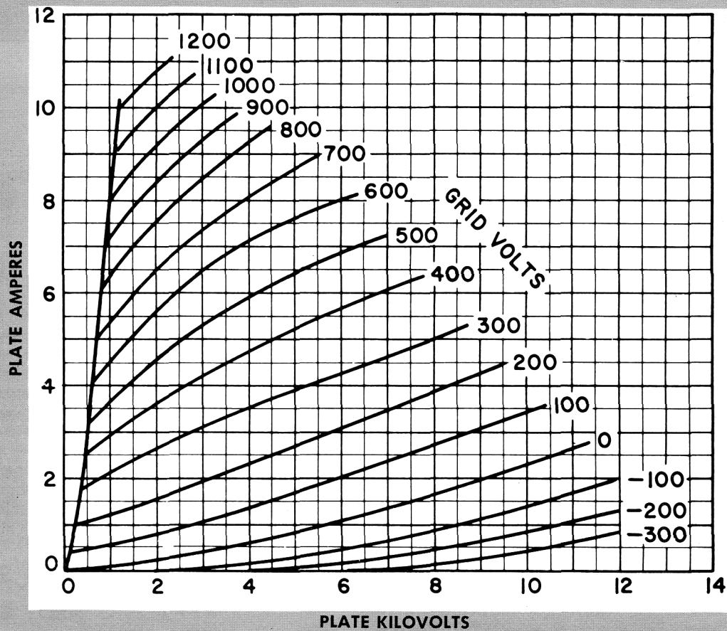
PLATE CHARACTERISTICS
