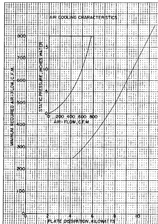
COOLING CHARACTERISTICS — ML-5669
