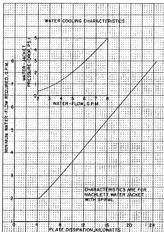
COOLING CHARACTERISTICS — ML-5668
