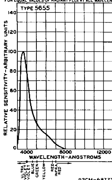
SPECTRAL SENSITIVITY CHARACTERISTIC FOR EQUAL VALUES OF RADIANT FLUX AT ALL WAVELENGTHS
