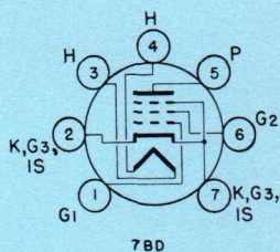
BOTTOM VIEW BASING DIAGRAM JEDEC 7BD
