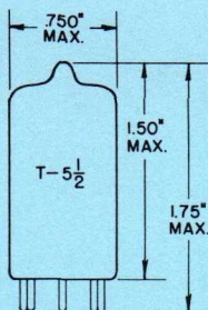
GLASS BULB SMALL-BUTTON MINIATURE 7 PIN BASE E7-1
