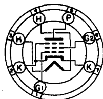
BOTTOM VIEW MINIATURE BUTTON 7 PIN BASE 780
