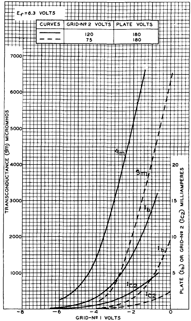
Fig. 2 - Average Characteristics of 5654.
