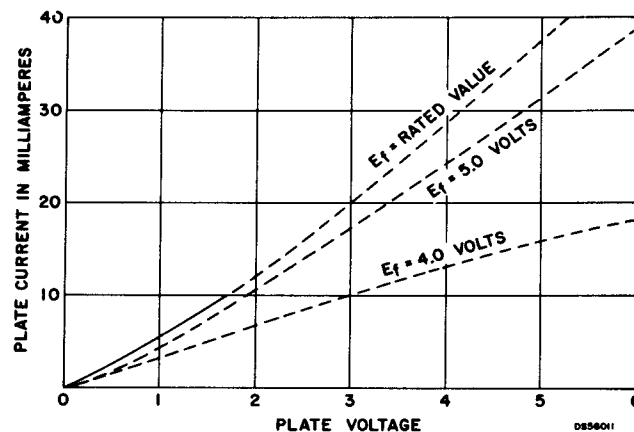
Figure 1—Approximate Plate Characteristics at reduced heater voltage.
