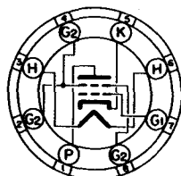
BOTTOM VIEW SUBMINIATURE BUTTON 8 FLEXIBLE LEADS .047" TINNED
