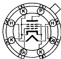
BOTTOM VIEW SUBMINIATURE BUTTON 8 PIN BASE
