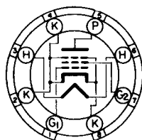
BOTTOM VIEW SUBMINIATURE BUTTON 8 FLEXIBLE LEADS 8DL
