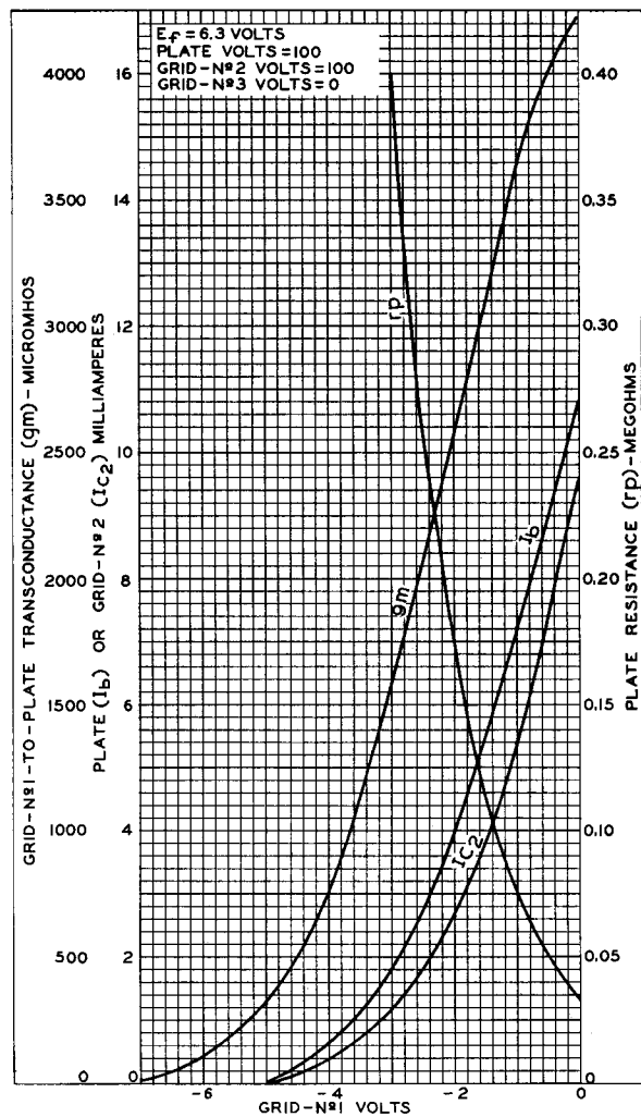
Fig.2 - Average Characteristics of Type 5636.
