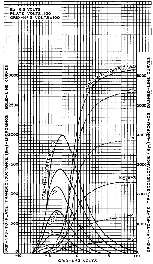
Fig.4 - Average Characteristics of Type 5636.
