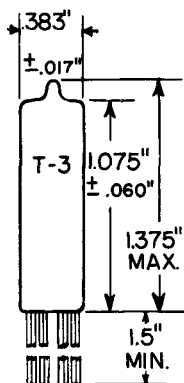
GLASS BULB
