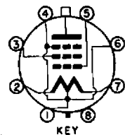
Terminal Layout
