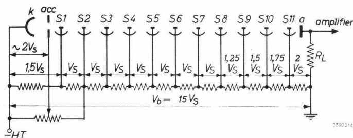
Voltage divider type B 3)
