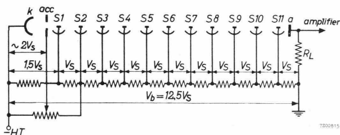
Voltage divider type A 3)
