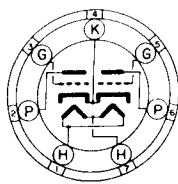
7B BOTTOM VIEW MEDIUM 7 PIN BASE
